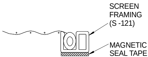
HEAD, JAMB 1 & SILL DETAIL SCALE: FULL HEAD AND SILL SIMILAR
